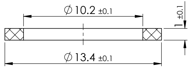
SECTION X-X
